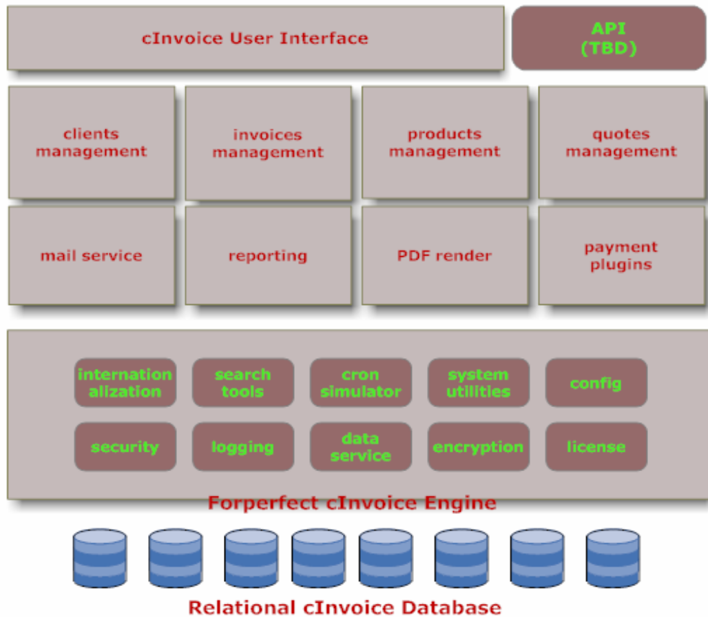
Figure 1: cInvoice system components
